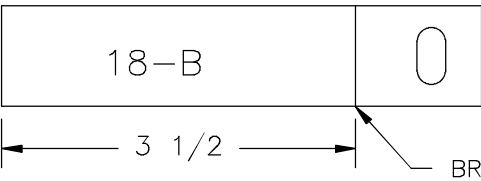
ITEM B MATL: FI 1/4 x 1 x 4-3/4 HRS 1 REQUIRED
